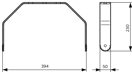
GreenPerform High-bay gen2 acc. BY698Z
